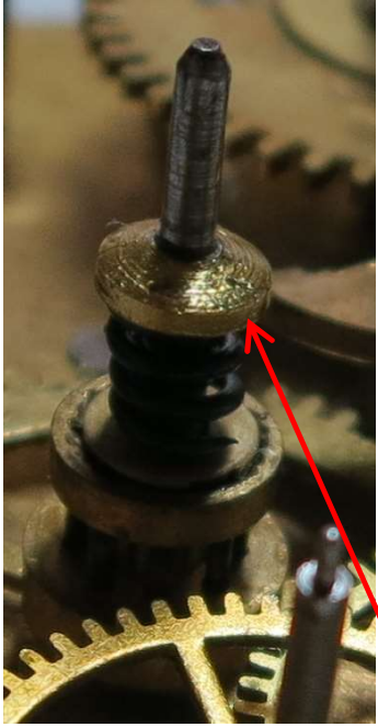
Second wheel compression washer Result = erratic, slow or no hand movement
